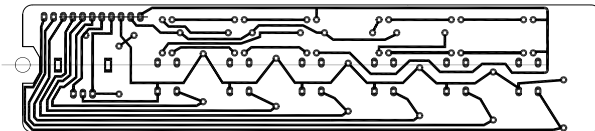
PCB BACK SIDE COPPER LAYER
