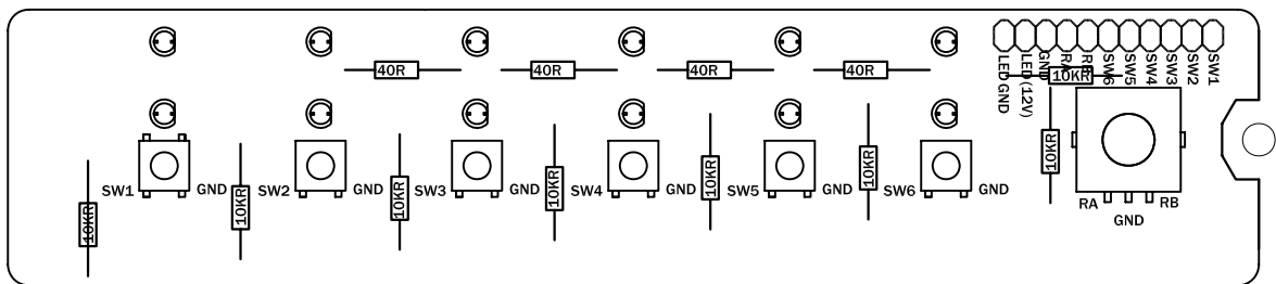
PCB – FRONT TEXT LAYER
